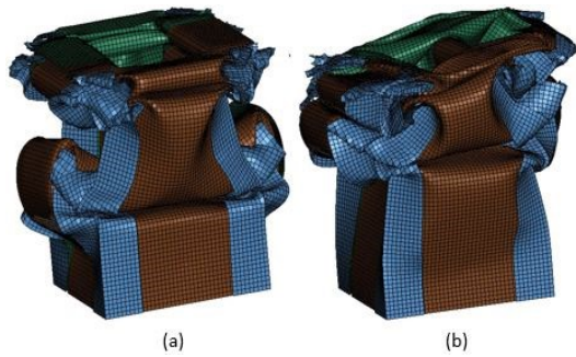
Figure 8. deformation mode of outside reinforcement model under (a) axial loading ( \theta = 0^\circ ), (b) oblique loading ( \theta = 10^\circ )
